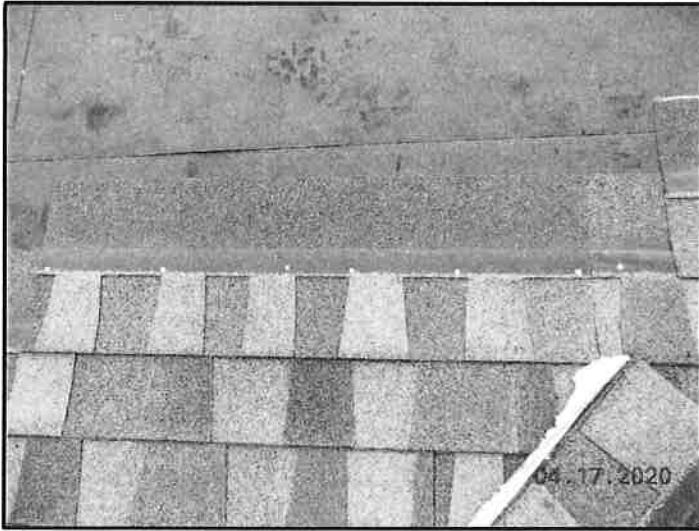
Shingle Nailing
