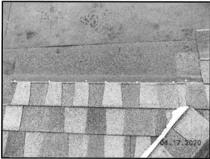
Shingle Nailing
