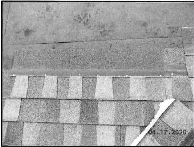
Shingle Nailing
